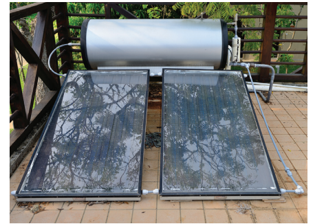
Solar Batch Heater
